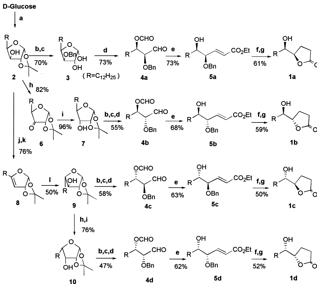
Scheme 1. Preparation of muricatacin 1a–d . (a) See reference 7 ; (b) NaH, BnCl, THF, rt, 5h; (c) 9.6 N HCl/TFA, DME, rt, 48h; (d) NaIO 4 , MeOH, rt, 1h; (e) NaH, (EtO) 2 POCH 2 CO 2 Et, THF, rt 3h; (f) H 2 , Pd-C, EtOAc, rt, 24h; (g) TFA-H 2 O (4:1), rt, 3h; (h) DMSO, (COCl) 2 , Et 3 N, CH 2 Cl 2 , -60°C→rt, 2h; (i) NaBH 4 , MeOH, rt; (j) Tf 2 O, pyridine, CH 2 Cl 2 , -10°C; (k) DBU, ether, rt; (l) Sia 2 BH, THF, 0°C→rt, then H 2 O 2 , aq. NaOH.
